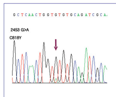
Exon 19 mut
